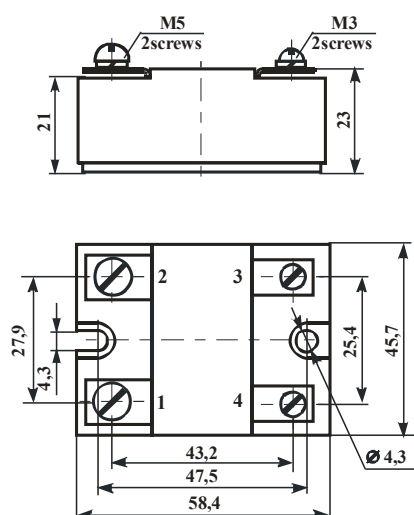
Figure 6.1 – Overall drawing of modules MO14, MO15D with maximum current up to 80 A
